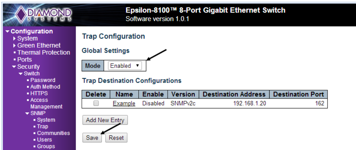
Figure 9 – Trap configuration
