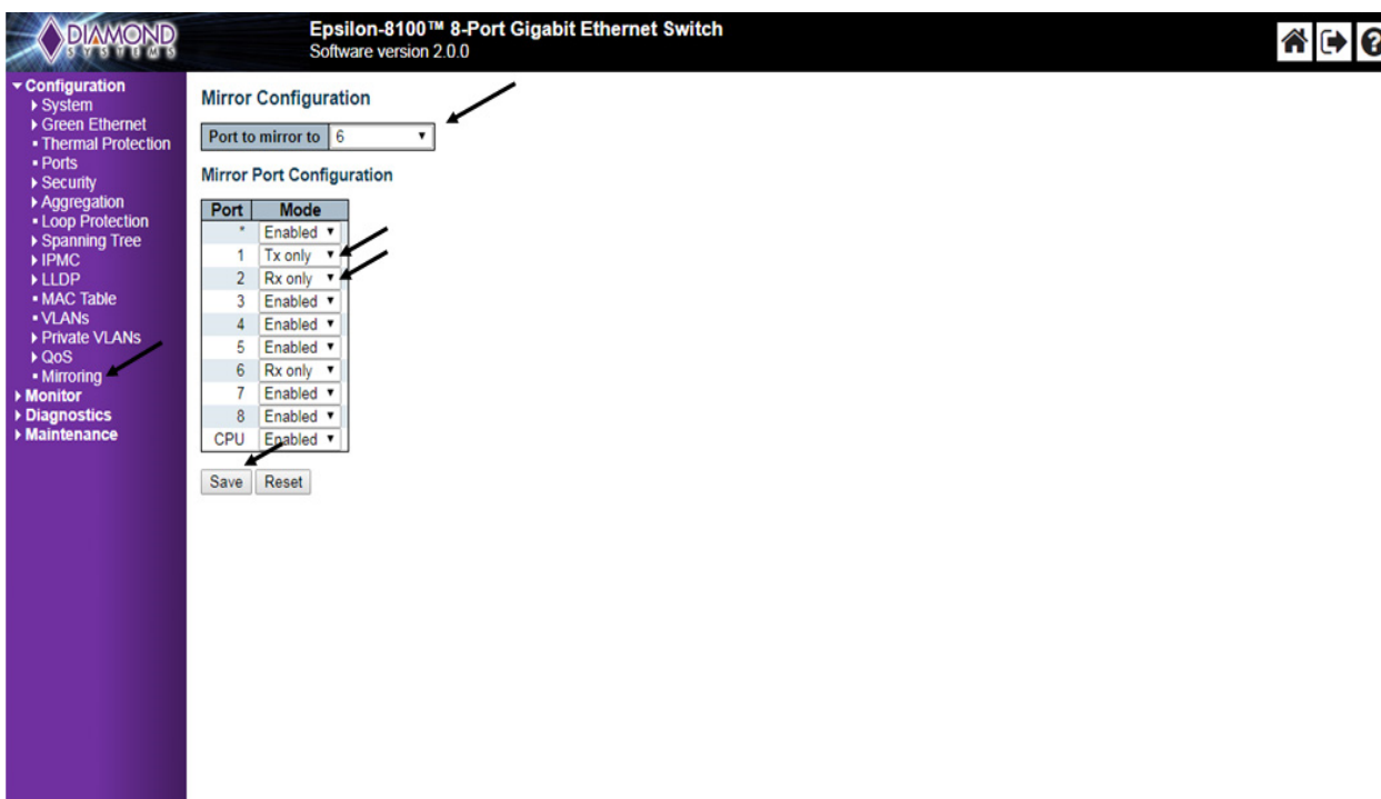
Figure 10 – Mirroring Configuration
